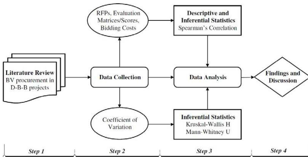
Fig. 1. Research methodology.
